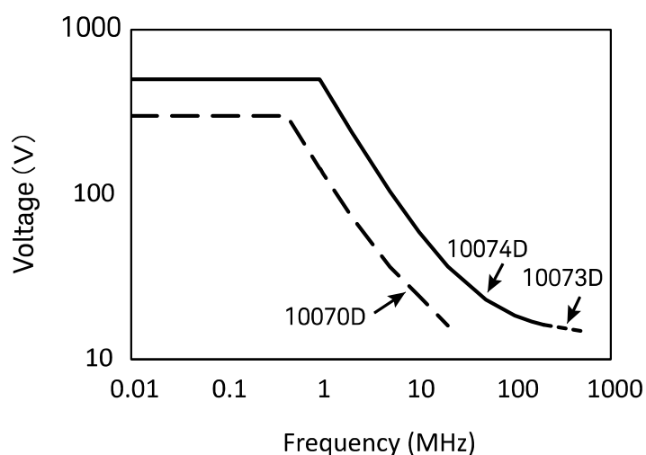
Derating Curve (Mains Isolated)
