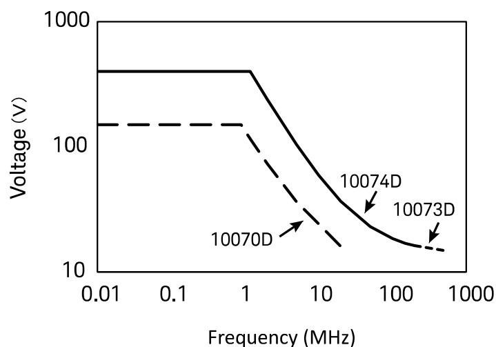
Derating Curve (CAT II)
