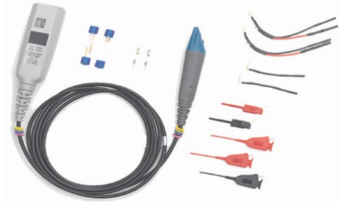
N2797A 1.5 GHz Single-ended active probe
