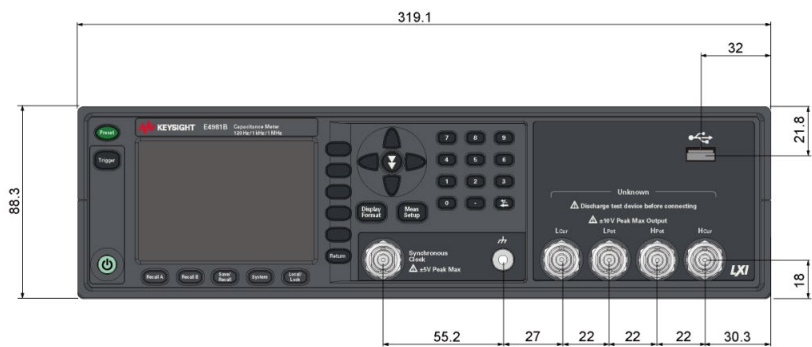
Figure 16. Dimensions (front view, without handle and bumper, in millimeters, nominal)
