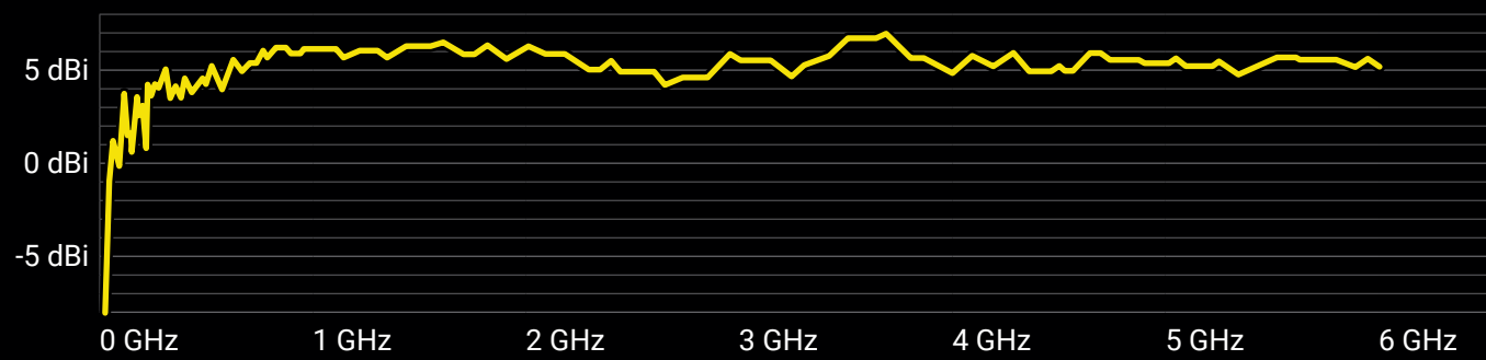
Gain Diagram HyperLOG® 20600 EMI (10 m)
