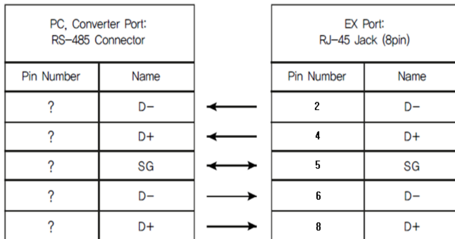
485 to 232 Converter
